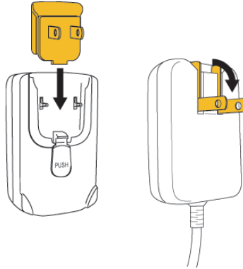
Figure 5. Insert plug attachment or fold plug blades down (if required)
